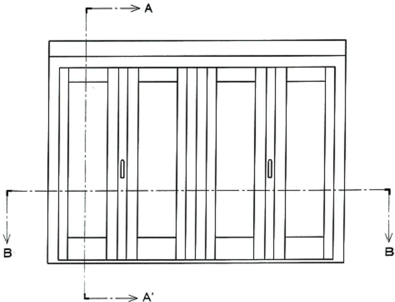
< Inside View >
