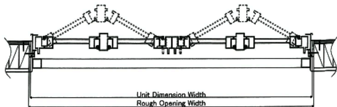
< B-B' Section >
