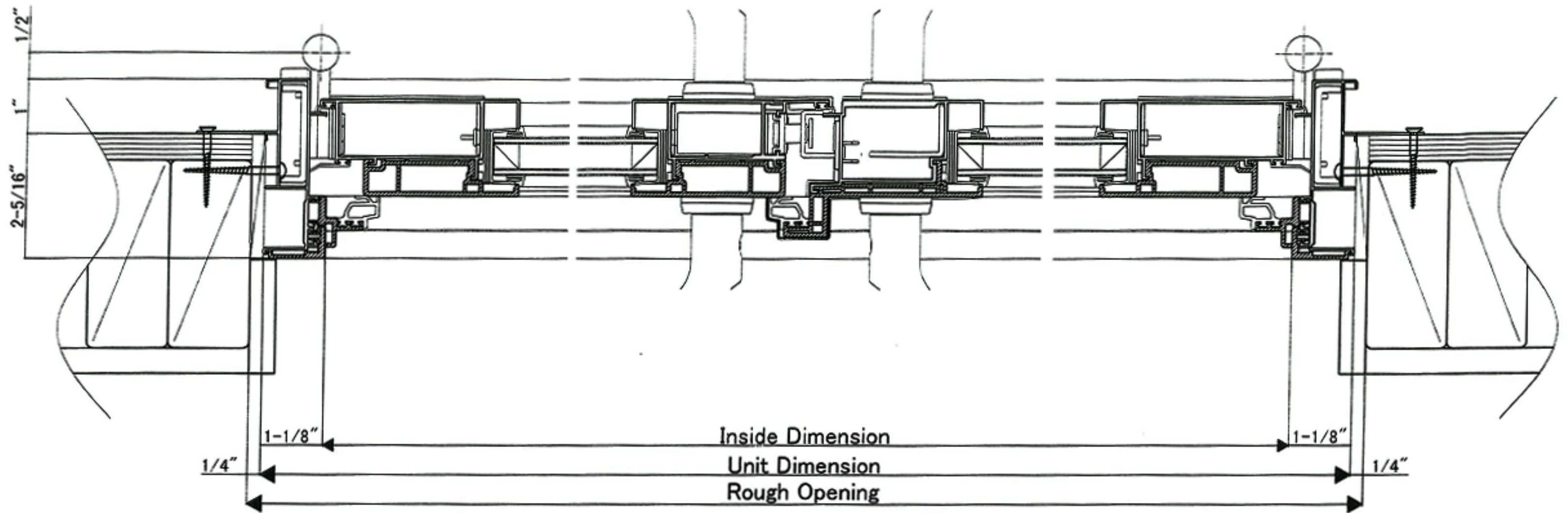
French Door (Double Leaf) 【Horizontal Drawing】
