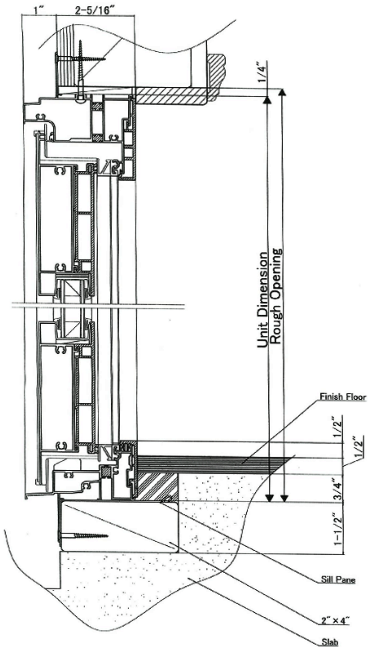
French Door (Double Leaf) 【Vertical Drawing】
