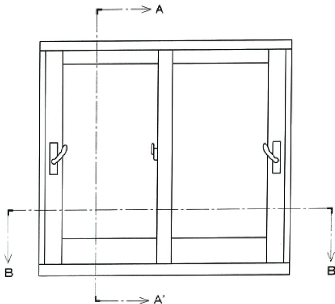
< Inside View >
