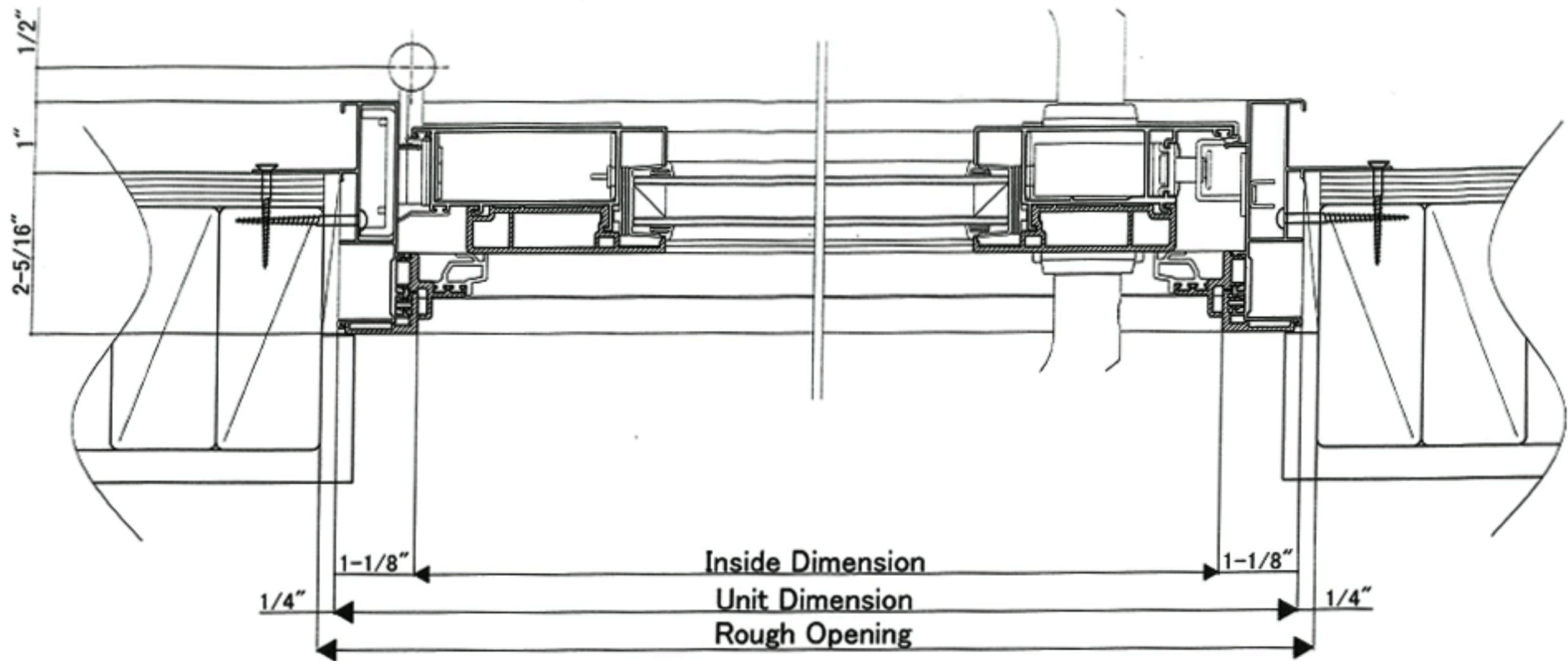
French Door (Single Leaf) ~Hinge Right~ 【Horizontal Drawing】
